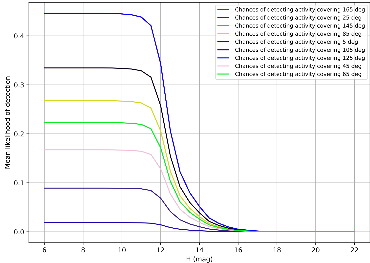
too_elab_heavy_r64_d2_gz_v3.4_10yrs OCC_r20
