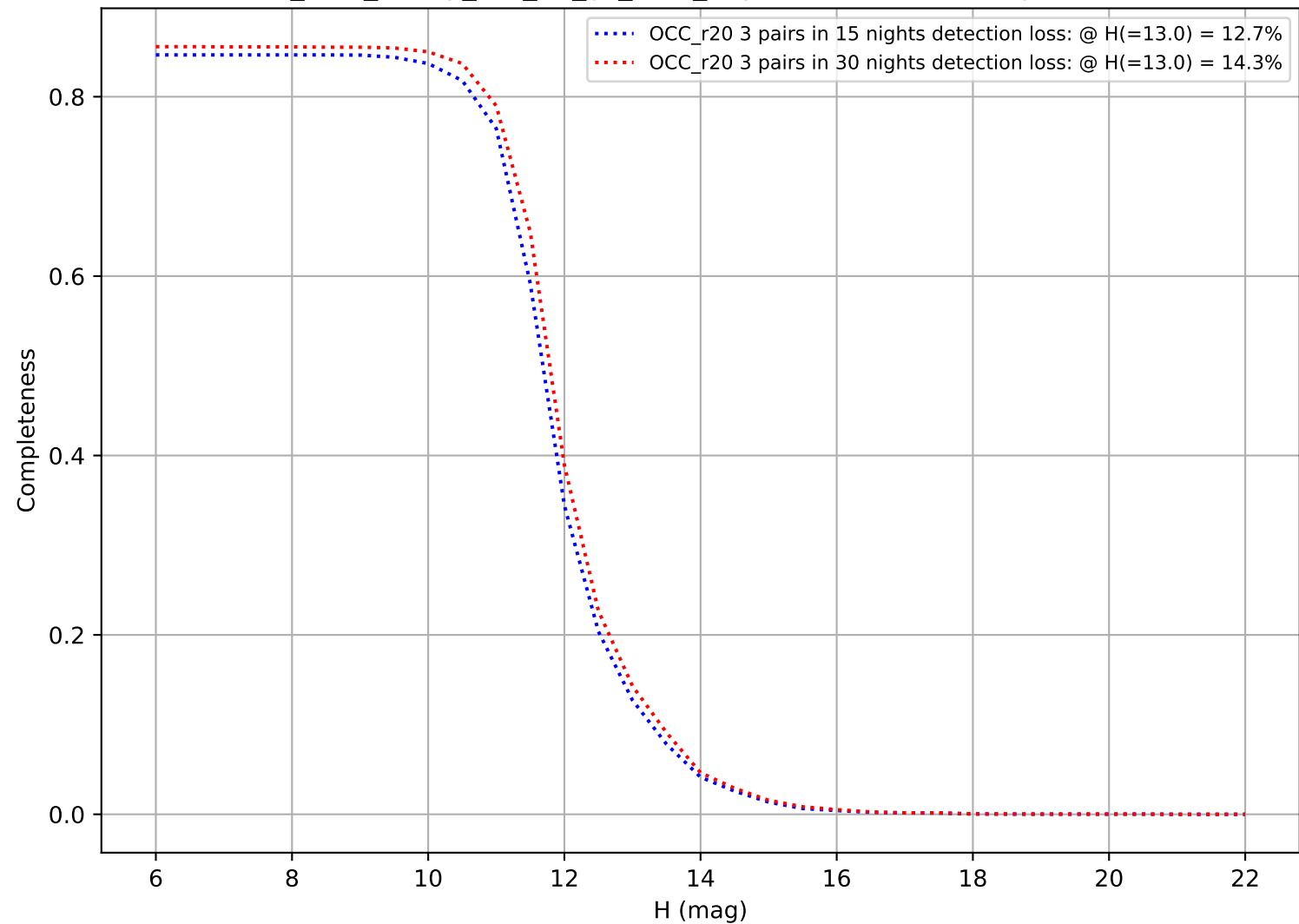
too_elab_heavy_r64_d2_gz_v3.4_10yrs: DifferentialCompleteness
