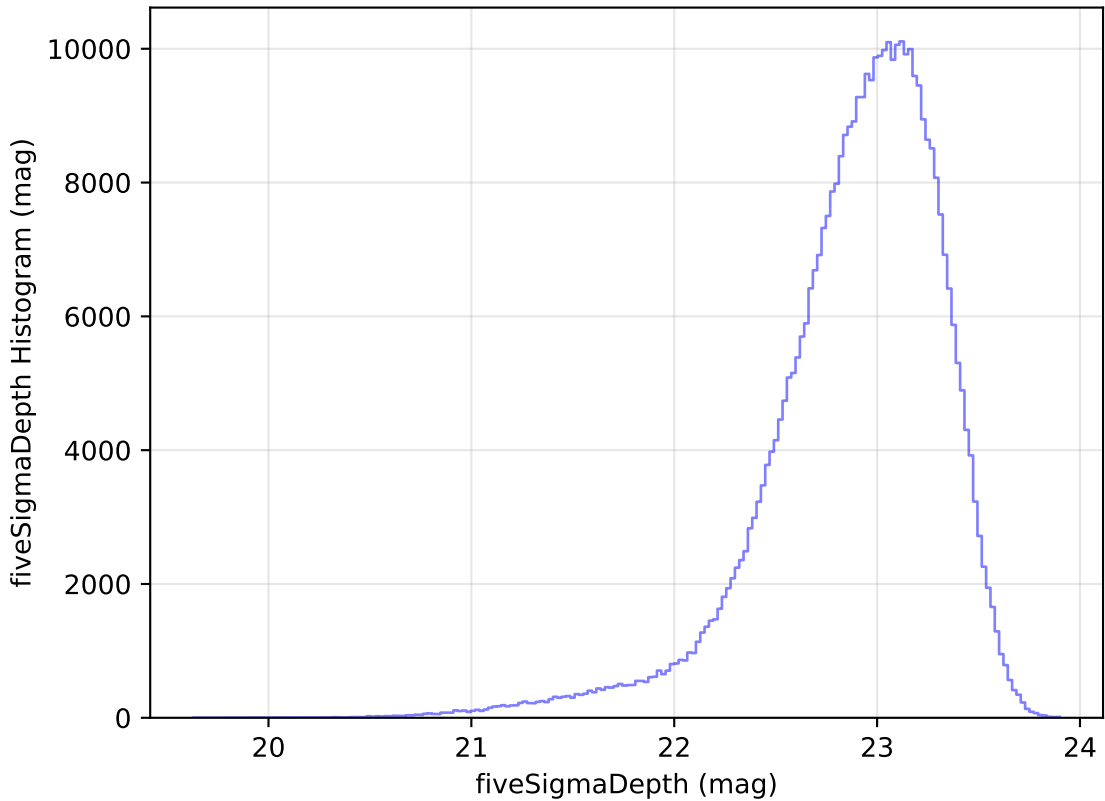
too_elab_heavy_r64_d2_gz_v3.4_10yrs z: fiveSigmaDepth Histogram
