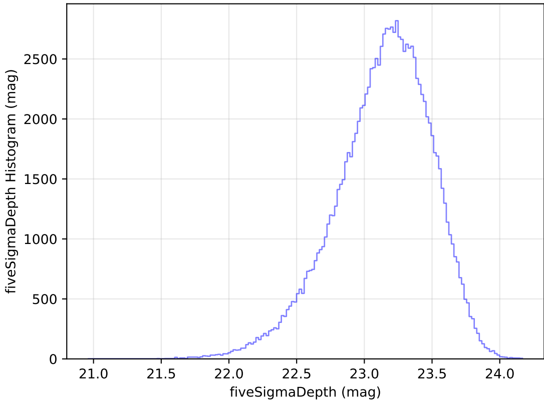
too_elab_heavy_r64_d2_gz_v3.4_10yrs u: fiveSigmaDepth Histogram
