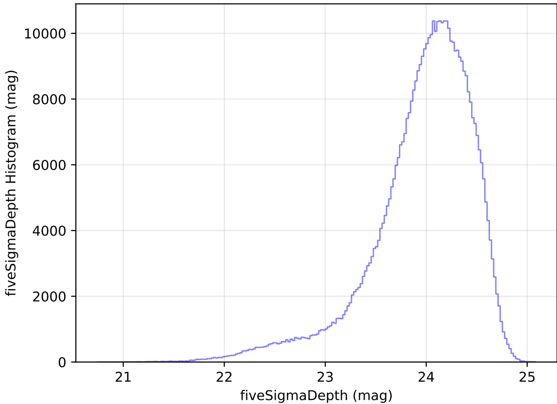
too_elab_heavy_r64_d2_gz_v3.4_10yrs r: fiveSigmaDepth Histogram
