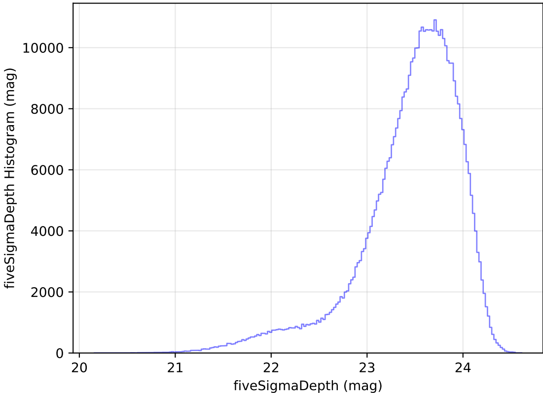
too_elab_heavy_r64_d2_gz_v3.4_10yrs i: fiveSigmaDepth Histogram
