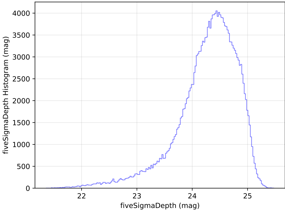
too_elab_heavy_r64_d2_gz_v3.4_10yrs g: fiveSigmaDepth Histogram
