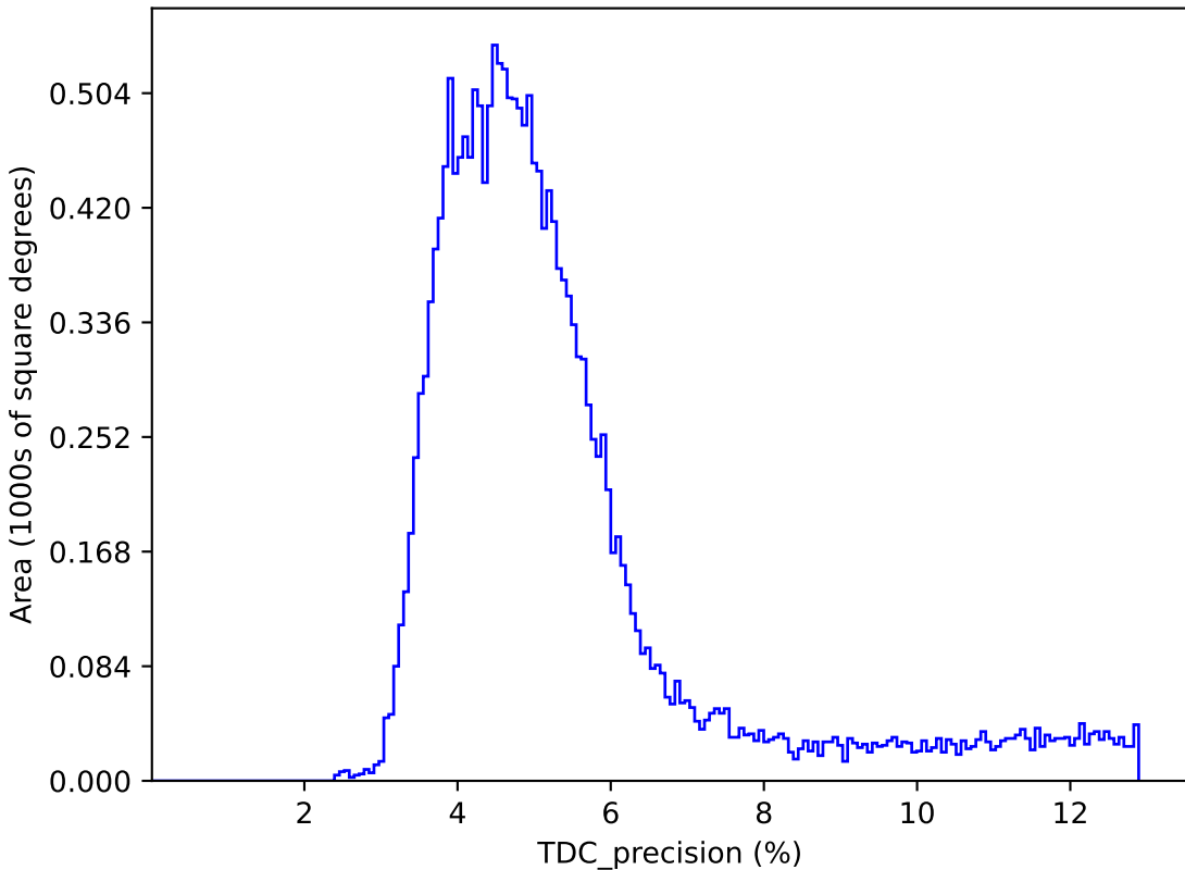
too_elab_heavy_r64_d2_gz_v3.4_10yrs : TDC_precision
