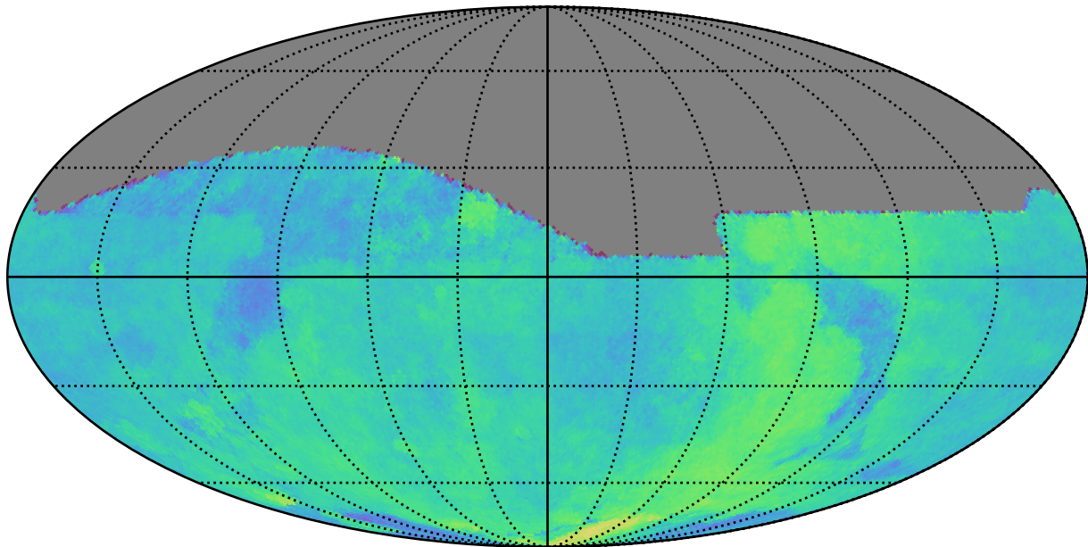
too_elab_heavy_r64_d2_gz_v3.4_10yrs : Parallax Coverage @ 24.0
