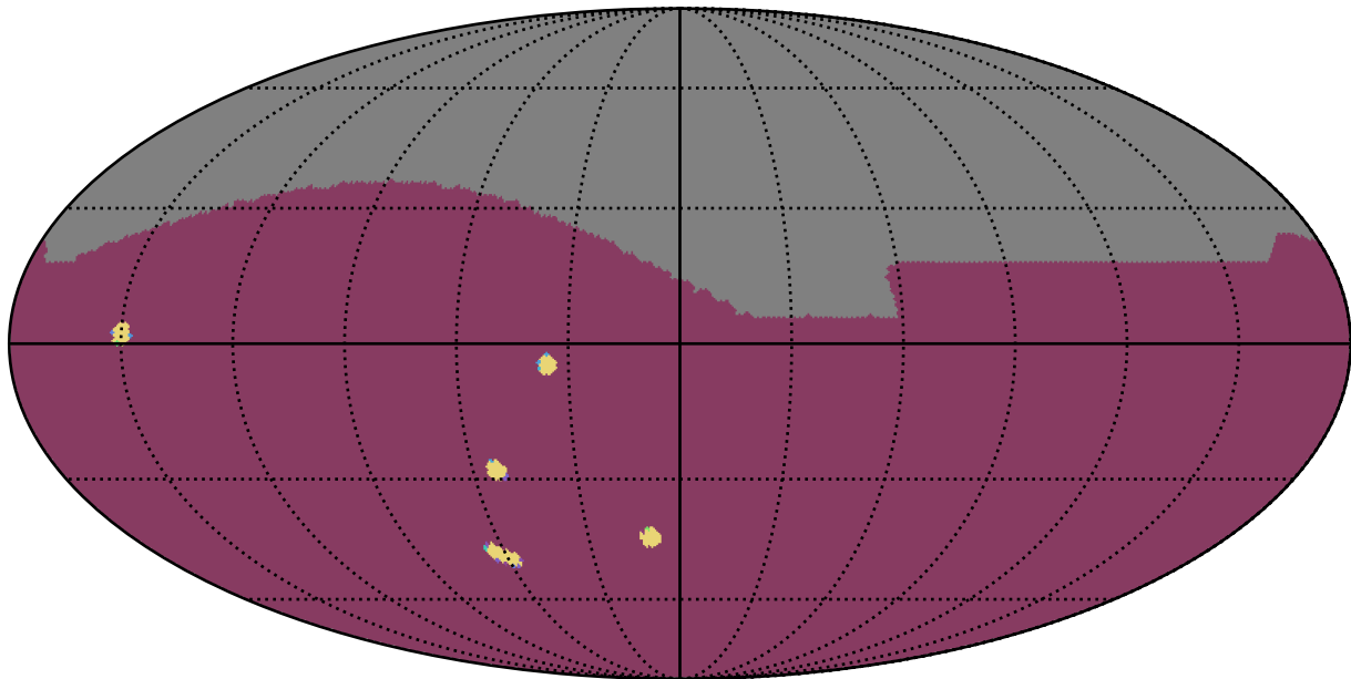
too_elab_heavy_r64_d2_gz_v3.4_10yrs : NumberOfQuickRevisits
