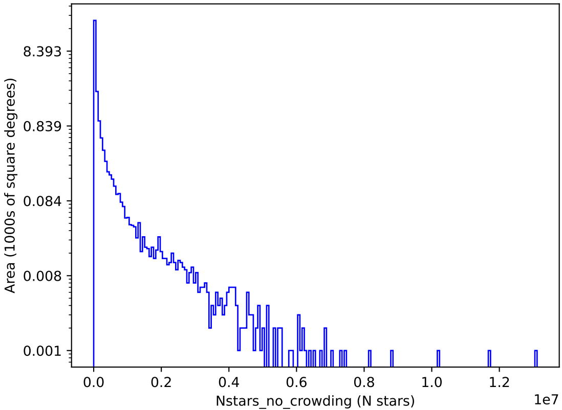
too_elab_heavy_r64_d2_gz_v3.4_10yrs g: Nstars_no_crowding
