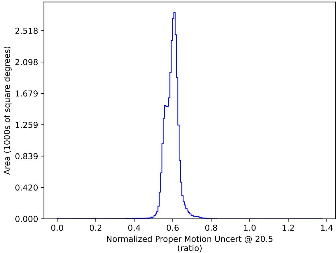
too_elab_heavy_r64_d2_gz_v3.4_10yrs : Normalized Proper Motion Uncert @ 20.5
