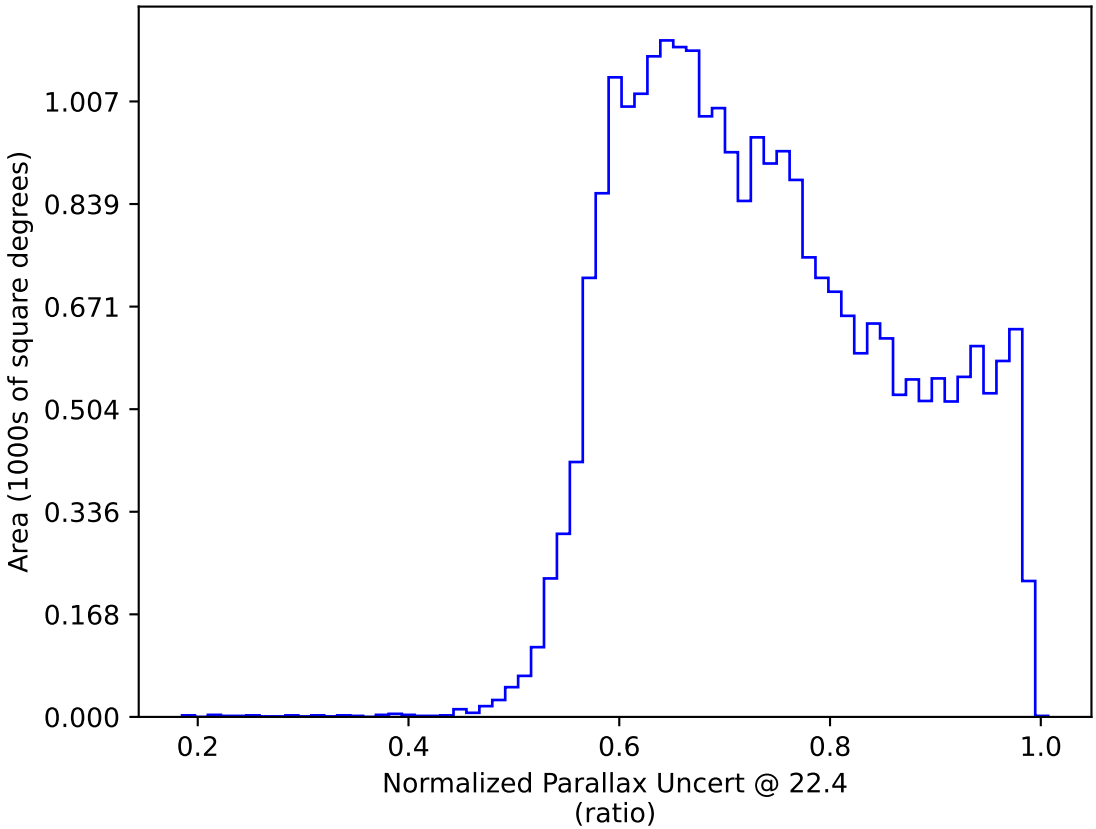
too_elab_heavy_r64_d2_gz_v3.4_10yrs : Normalized Parallax Uncert @ 22.4
