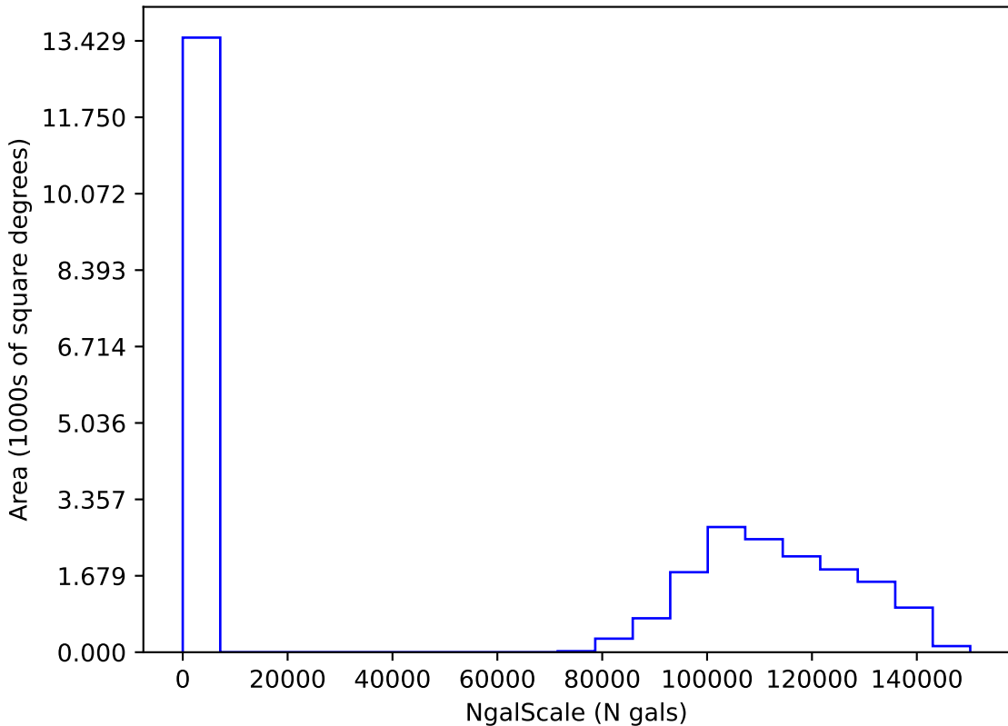
too_elab_heavy_r64_d2_gz_v3.4_10yrs i: NgalScale
