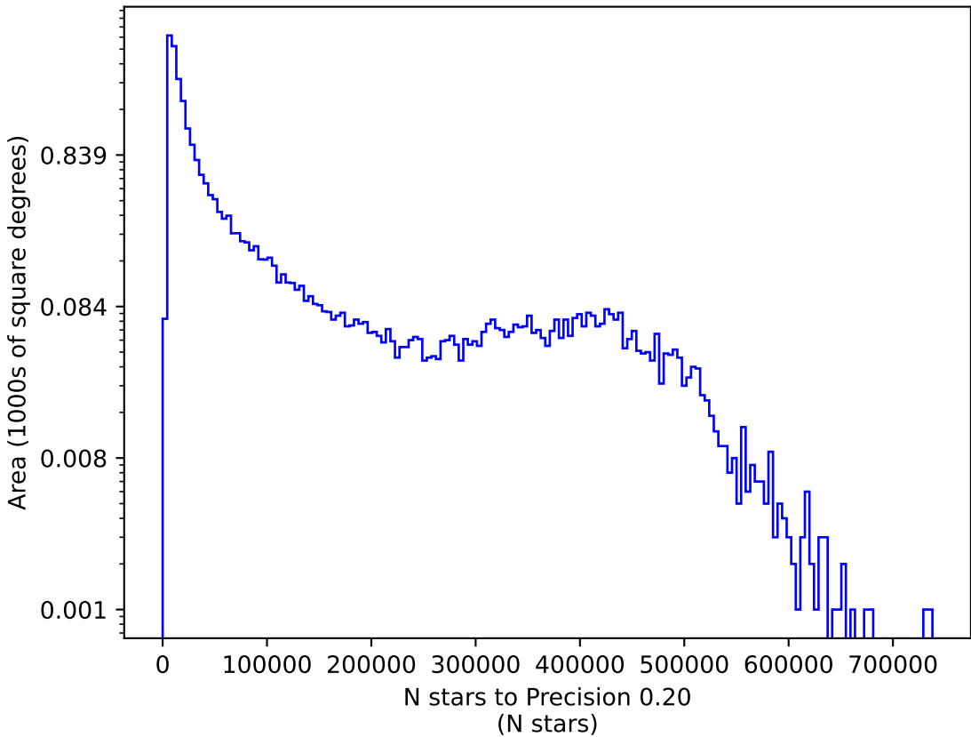
too_elab_heavy_r64_d2_gz_v3.4_10yrs r: N stars to Precision 0.20
