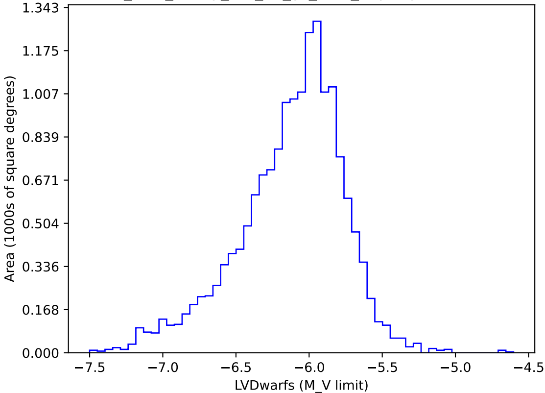
too_elab_heavy_r64_d2_gz_v3.4_10yrs gi: LVDwarfs
