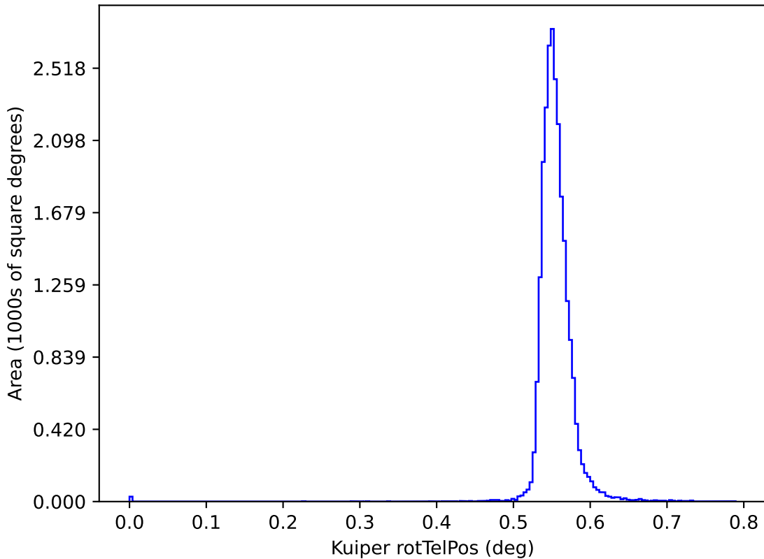
too_elab_heavy_r64_d2_gz_v3.4_10yrs y: Kuiper rotTelPos
