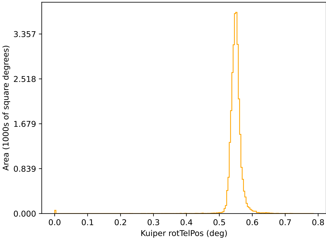
too_elab_heavy_r64_d2_gz_v3.4_10yrs r: Kuiper rotTelPos
