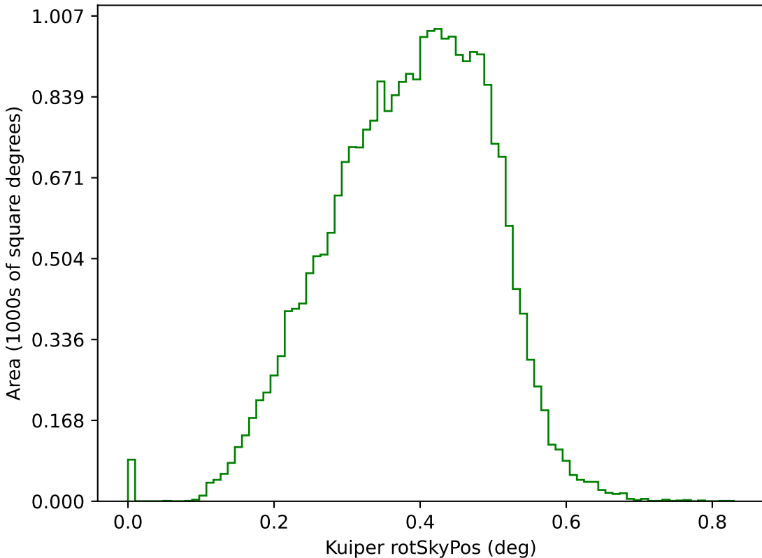
too_elab_heavy_r64_d2_gz_v3.4_10yrs g: Kuiper rotSkyPos
