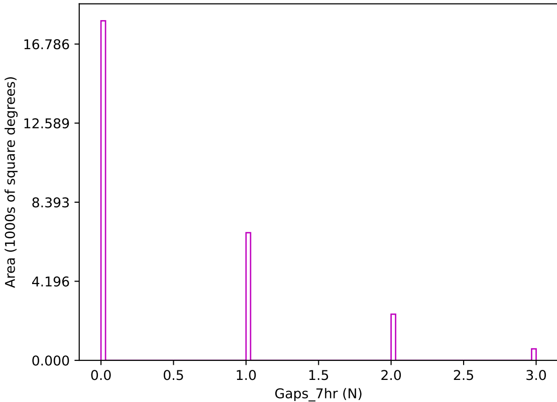
too_elab_heavy_r64_d2_gz_v3.4_10yrs z band: Gaps_7hr
