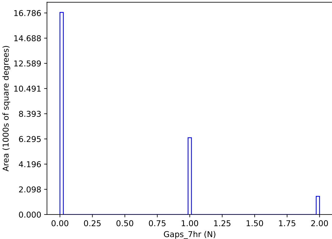
too_elab_heavy_r64_d2_gz_v3.4_10yrs y band: Gaps_7hr
