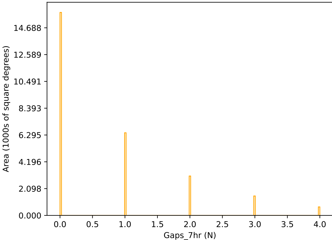
too_elab_heavy_r64_d2_gz_v3.4_10yrs r band: Gaps_7hr
