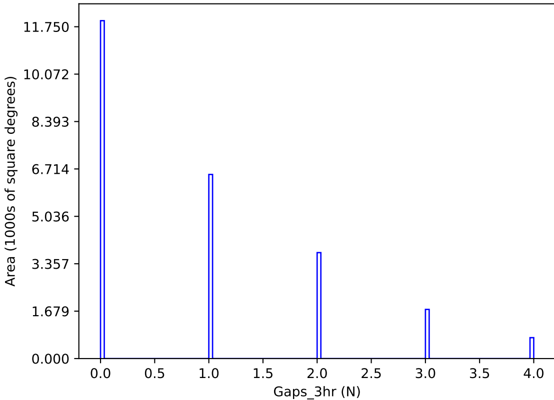
too_elab_heavy_r64_d2_gz_v3.4_10yrs y band: Gaps_3hr
