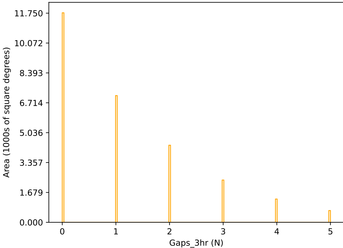
too_elab_heavy_r64_d2_gz_v3.4_10yrs r band: Gaps_3hr
