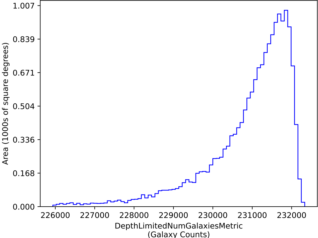
too_elab_heavy_r64_d2_gz_v3.4_10yrs i band galaxies non-DD: DepthLimitedNumGalaxiesMetric
