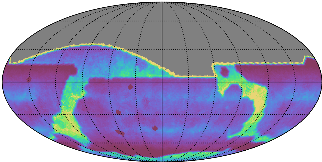
too_elab_heavy_r64_d2_gz_v3.4_10yrs : DCRprecision
