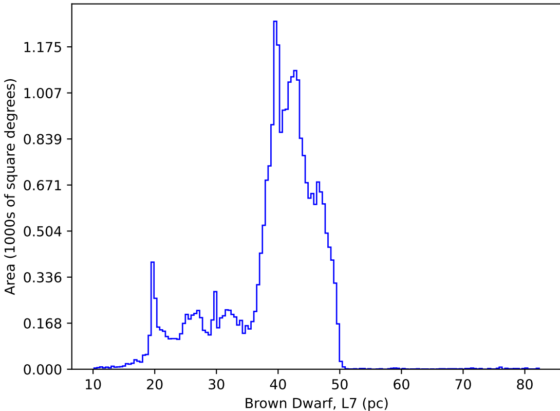
too_elab_heavy_r64_d2_gz_v3.4_10yrs : Brown Dwarf, L7
