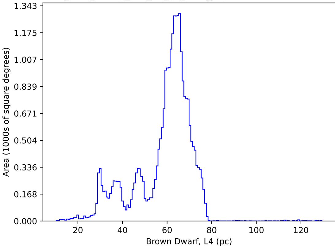
too_elab_heavy_r64_d2_gz_v3.4_10yrs : Brown Dwarf, L4
