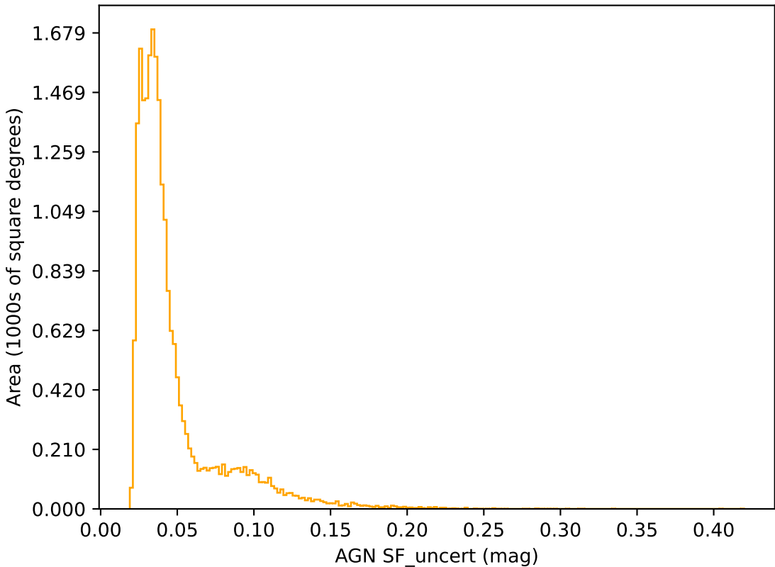
too_elab_heavy_r64_d2_gz_v3.4_10yrs r band: AGN SF_uncert
