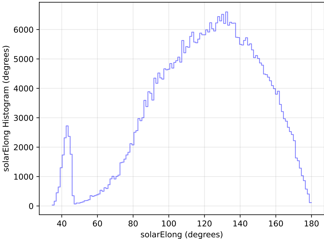
too_elab_heavy_r64_d2_gz_v3.4_10yrs WFD z band: solarElong Histogram
