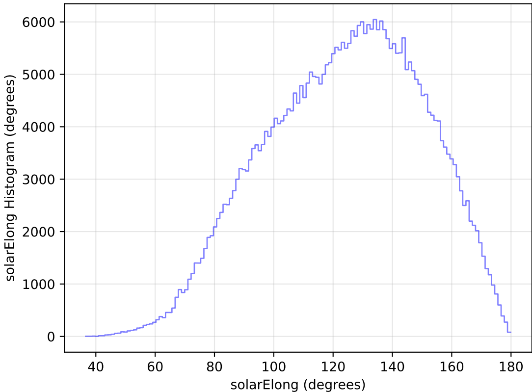
too_elab_heavy_r64_d2_gz_v3.4_10yrs WFD y band: solarElong Histogram
