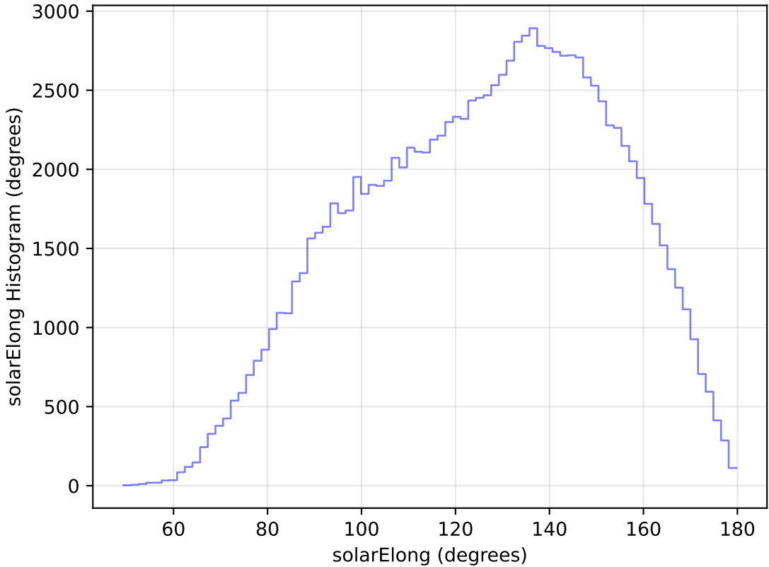
too_elab_heavy_r64_d2_gz_v3.4_10yrs WFD u band: solarElong Histogram
