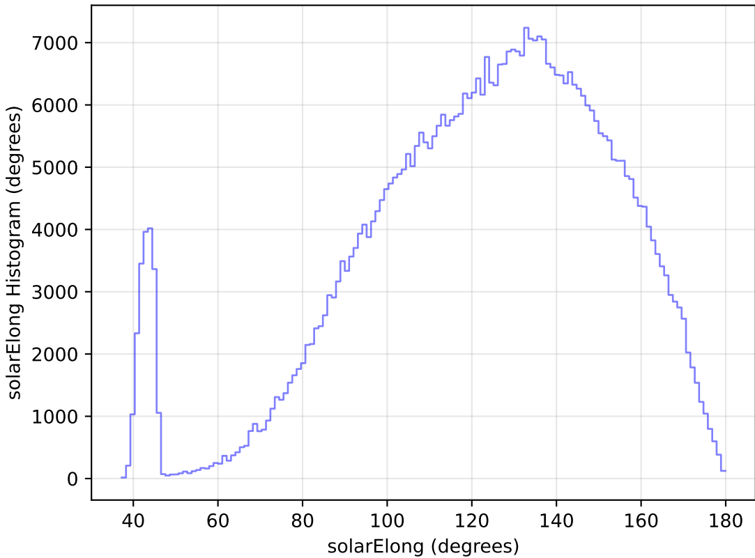
too_elab_heavy_r64_d2_gz_v3.4_10yrs WFD r band: solarElong Histogram
