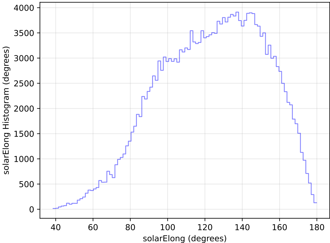
too_elab_heavy_r64_d2_gz_v3.4_10yrs WFD g band: solarElong Histogram
