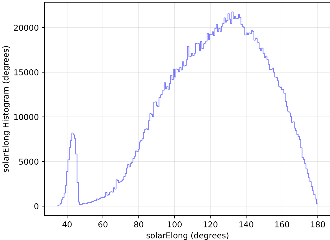
too_elab_heavy_r64_d2_gz_v3.4_10yrs WFD all bands: solarElong Histogram
