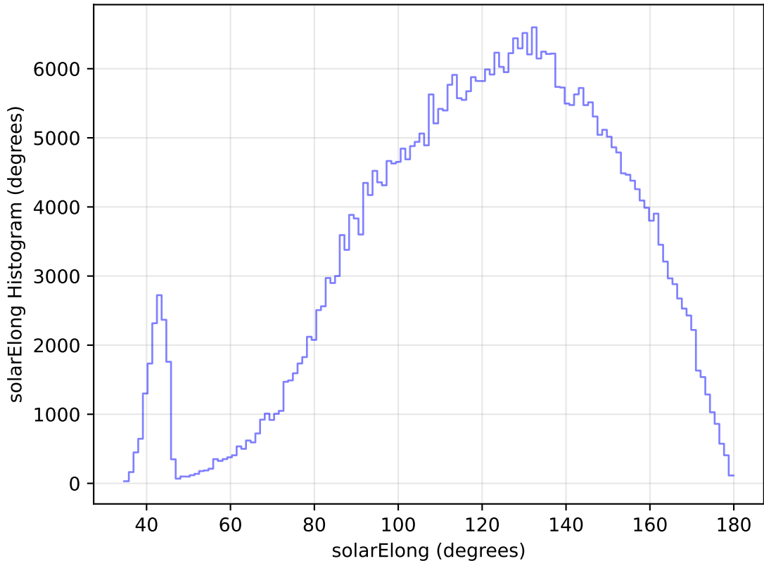
too_elab_heavy_r64_d2_gz_v3.4_10yrs All sky z band: solarElong Histogram
