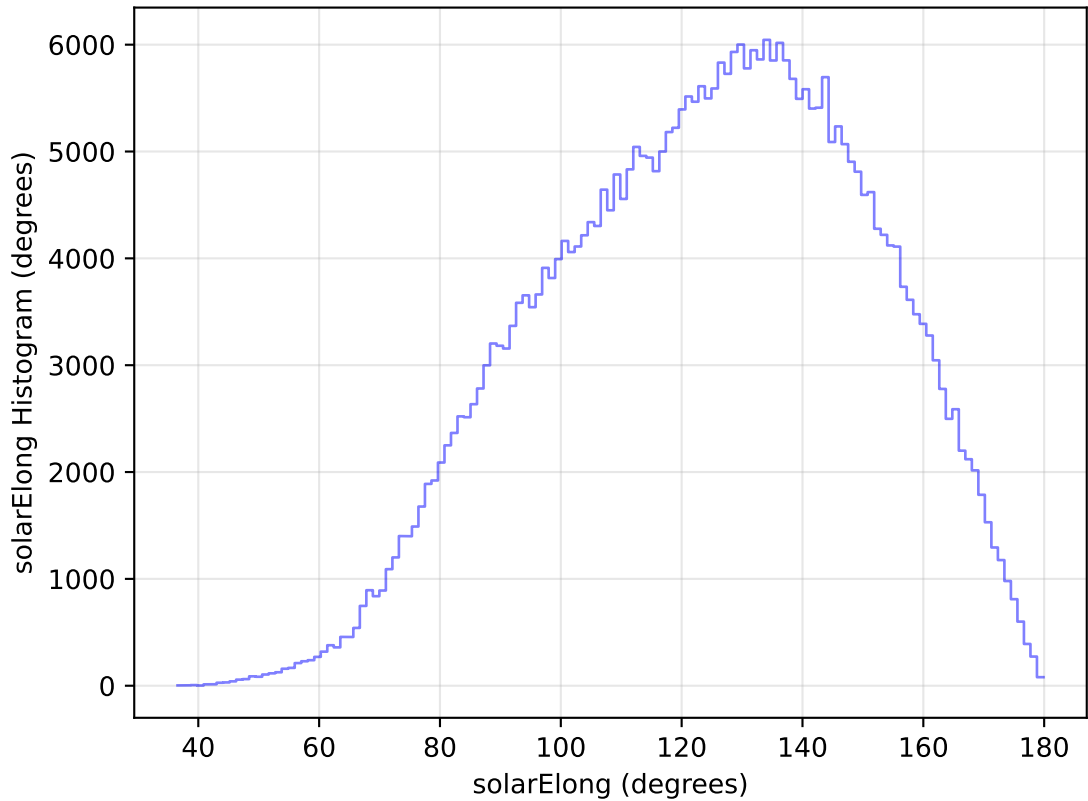
too_elab_heavy_r64_d2_gz_v3.4_10yrs All sky y band: solarElong Histogram
