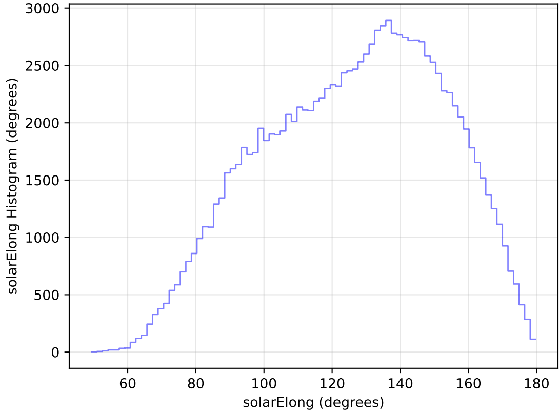
too_elab_heavy_r64_d2_gz_v3.4_10yrs All sky u band: solarElong Histogram
