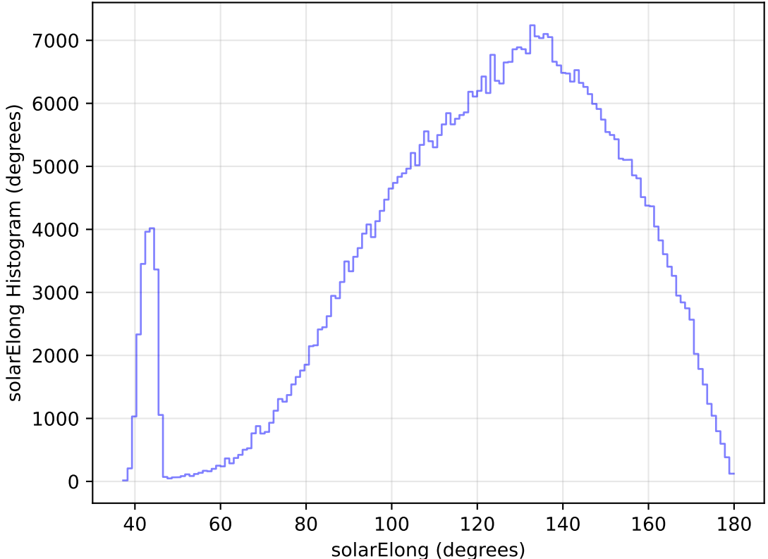
too_elab_heavy_r64_d2_gz_v3.4_10yrs All sky r band: solarElong Histogram
