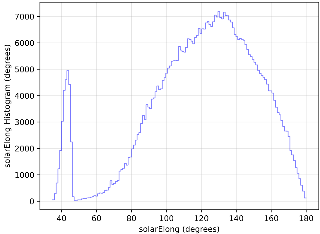
too_elab_heavy_r64_d2_gz_v3.4_10yrs All sky i band: solarElong Histogram
