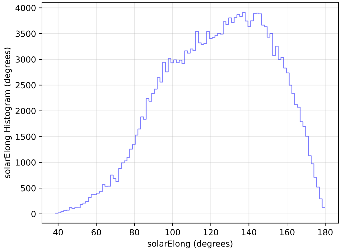
too_elab_heavy_r64_d2_gz_v3.4_10yrs All sky g band: solarElong Histogram
