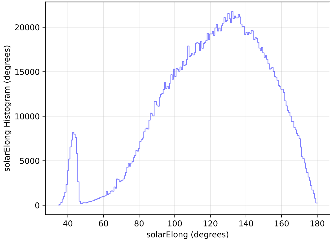
too_elab_heavy_r64_d2_gz_v3.4_10yrs All sky all bands: solarElong Histogram
