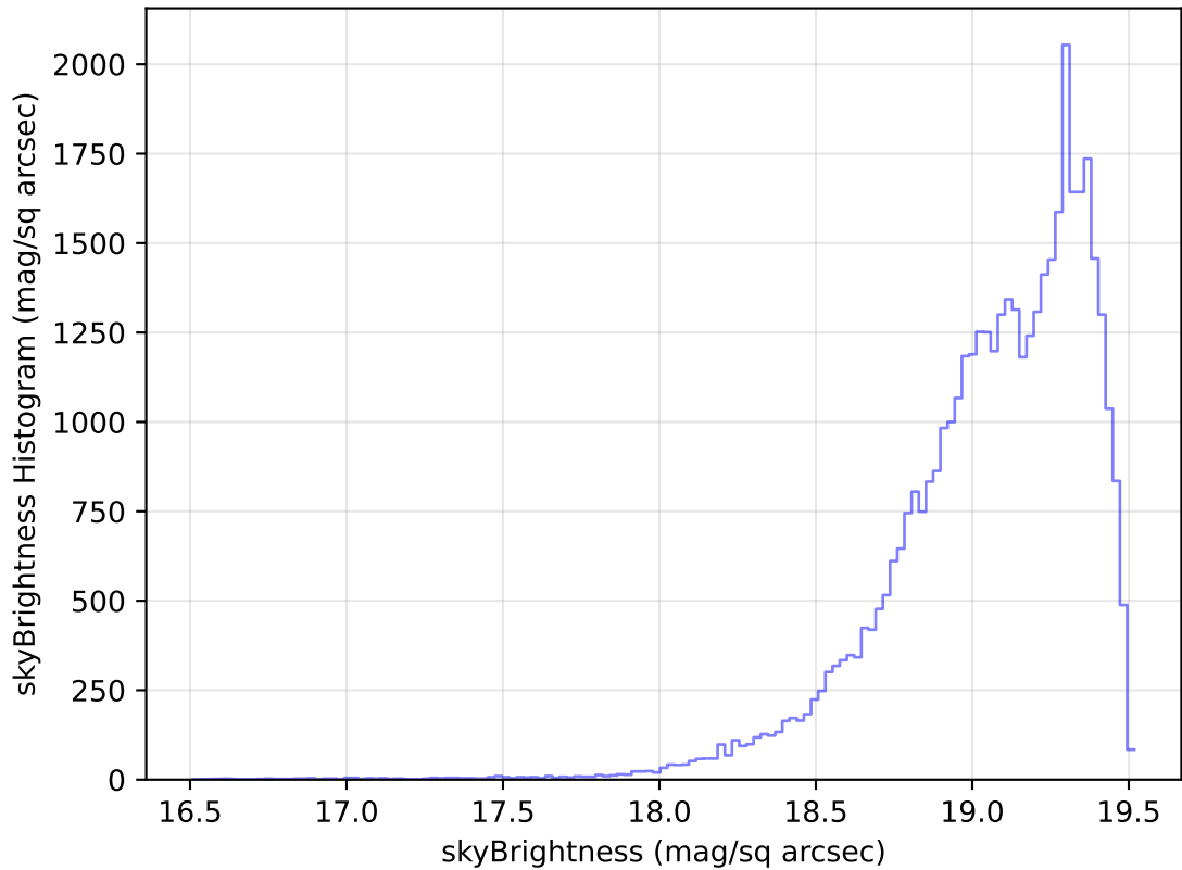
too_elab_heavy_r64_d2_gz_v3.4_10yrs Yr 1 z band: skyBrightness Histogram
