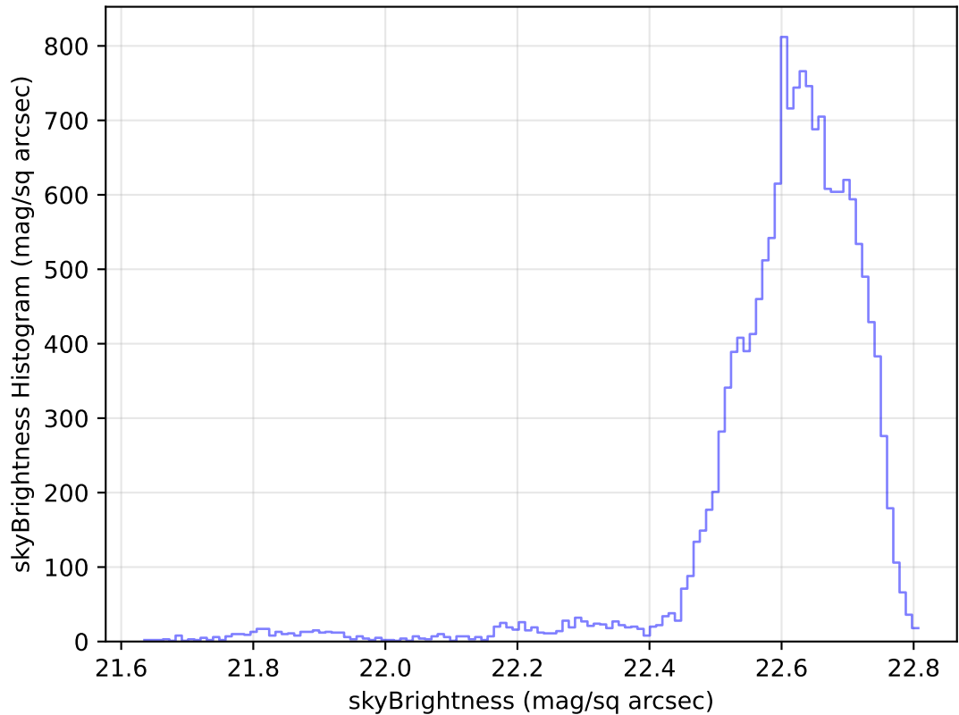
too_elab_heavy_r64_d2_gz_v3.4_10yrs Yr 1 u band: skyBrightness Histogram
