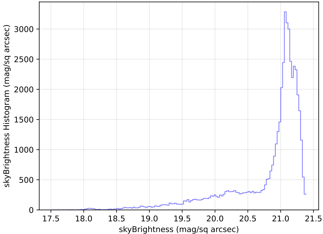
too_elab_heavy_r64_d2_gz_v3.4_10yrs Yr 1 r band: skyBrightness Histogram
