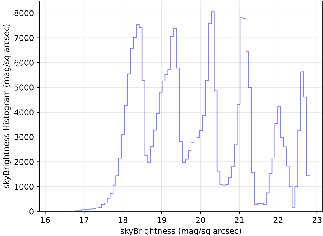
too_elab_heavy_r64_d2_gz_v3.4_10yrs Yr 1 all bands: skyBrightness Histogram
