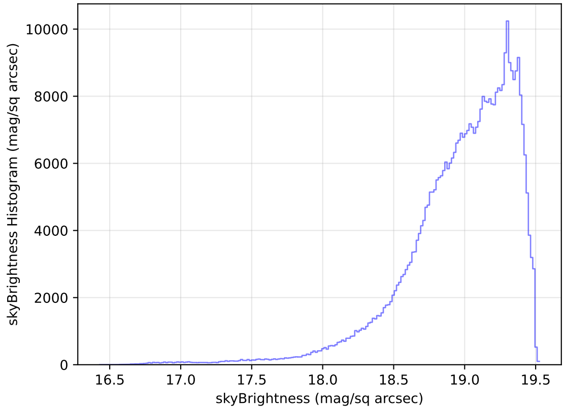
too_elab_heavy_r64_d2_gz_v3.4_10yrs WFD z band: skyBrightness Histogram
