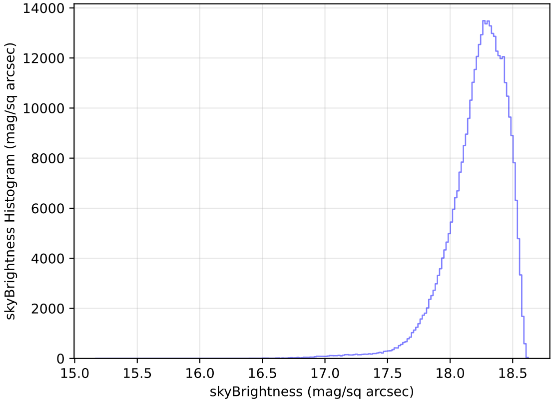
too_elab_heavy_r64_d2_gz_v3.4_10yrs WFD y band: skyBrightness Histogram
