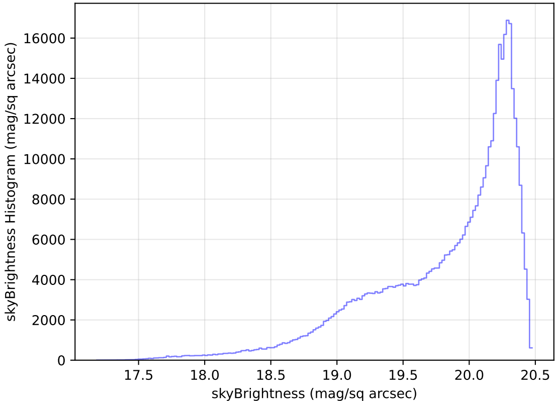
too_elab_heavy_r64_d2_gz_v3.4_10yrs WFD i band: skyBrightness Histogram
