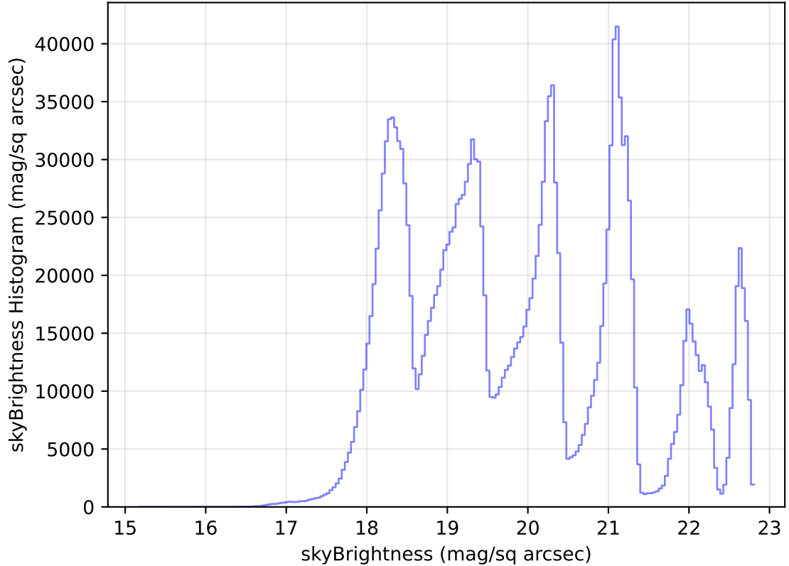
too_elab_heavy_r64_d2_gz_v3.4_10yrs WFD all bands: skyBrightness Histogram
